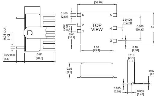
SMD- PACKAGE
